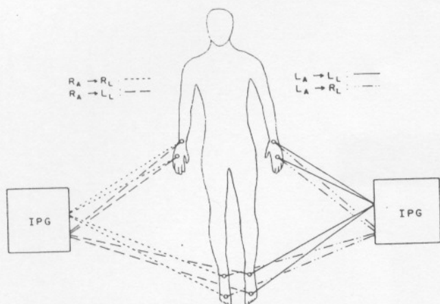
Fig. 1. Diagram of electrode arrangements used with the tetrapolar impedance plethysmograph (IPG). R = right, L = left, A = arm, L = leg.
